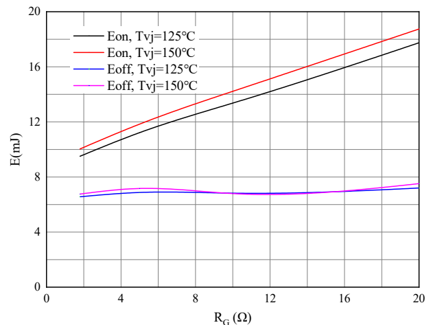
图 6. 开关损耗 逆变器 Figure 6. Switching losses of IGBT V_{GE}=\pm 15V, I_C=50A, V_{CE}=600V
